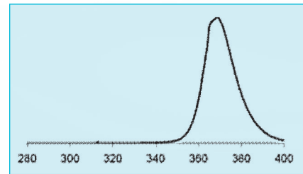
UVA-1
