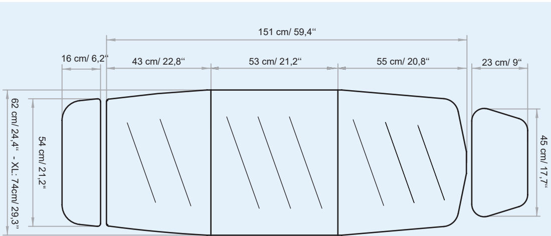
FLAT BI-ZAK
