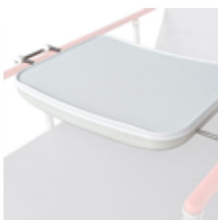
Universal Meal tray Extensible meal tray for side rails: from 65 to 88 cm Fall protection side Compatible with standardized tray meal : GastroNorm – GN1/1 : 53 x 32.5 cm EuroNorm : 53 x 37 cm It fits with all width of products. Maximum load: 10Kg PRU
