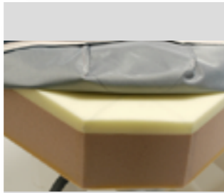
High Comfort mattress, high quality foam (35kg/m 3 ), 2cm thick viscoelastic layer (total thickness : 12cm) MMM
