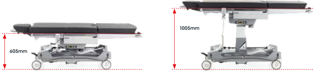
Patient platform height raise and lower
